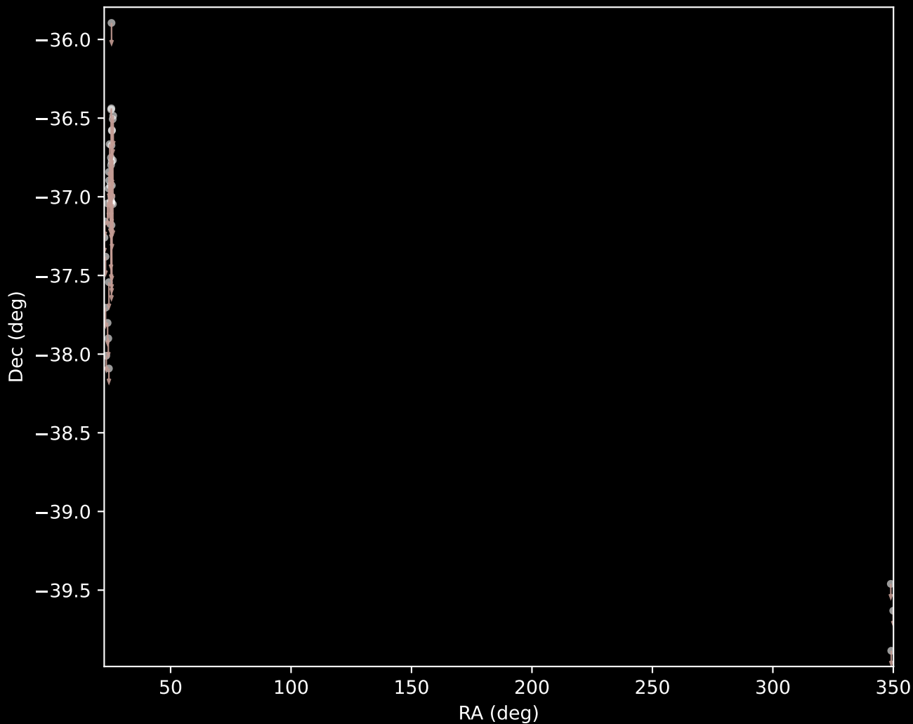
GALAH DR4 Cluster 111 Proper Motion Vectors (n=38)
