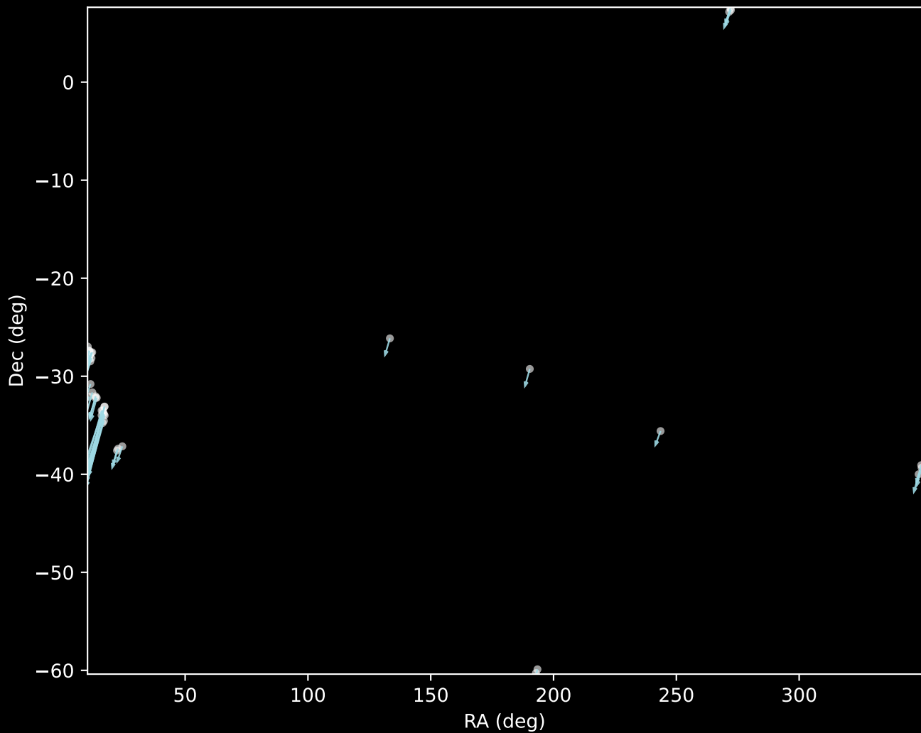
GALAH DR4 Cluster 379 Proper Motion Vectors (n=40)
