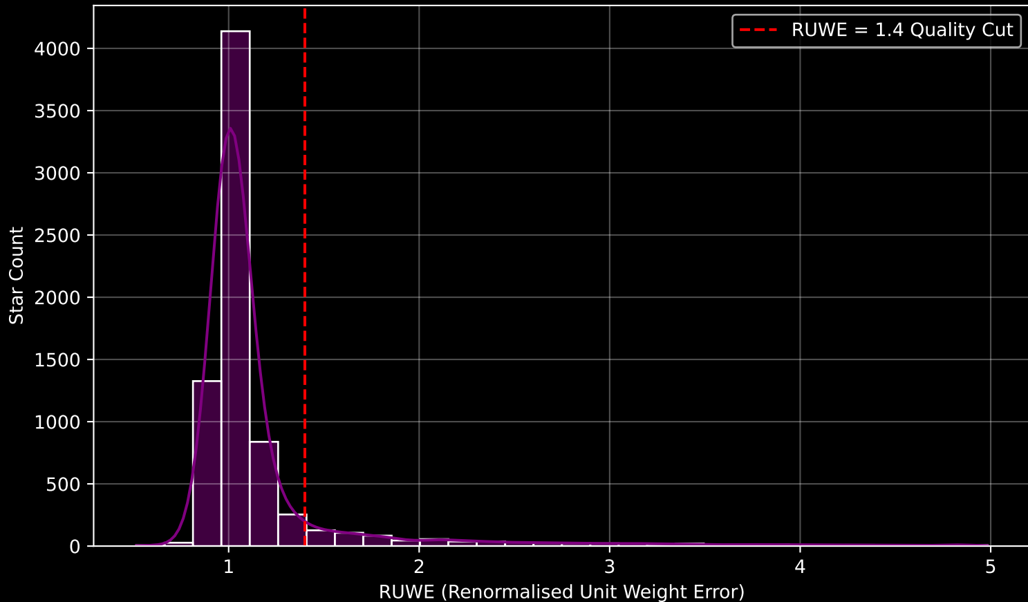
GALAH DR4 Field [-1] RUWE Distribution (n= 7330)
