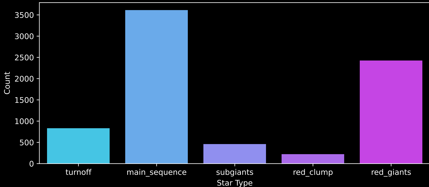
GALAH DR4 Field: [-1] Count plot of Star Type
