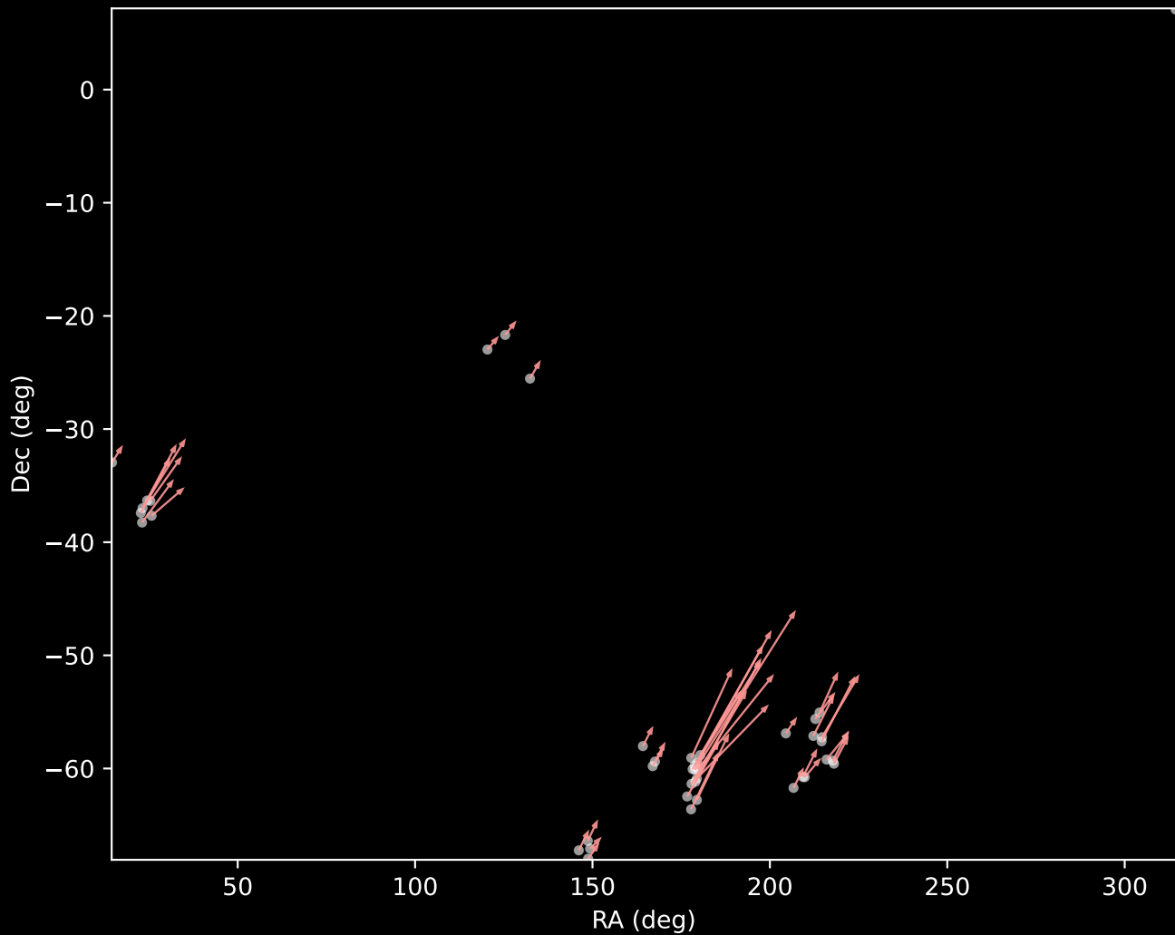
GALAH DR4 Cluster 267 Proper Motion Vectors (n=43)
