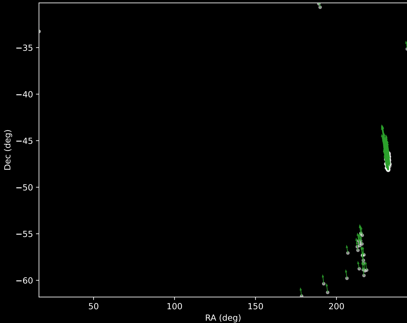
GALAH DR4 Cluster 424 Proper Motion Vectors (n=133)
