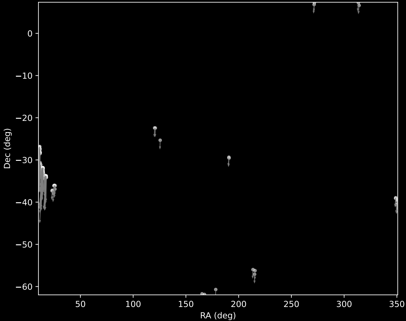
GALAH DR4 Cluster 394 Proper Motion Vectors (n=104)
